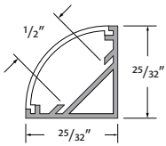
MRSL-CHAN-SLV-6.5 Anodized aluminum extrusion available in 6.5' length
