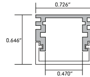
ASTR-CHAN-SLV-6.5 Anodized aluminum extrusion available in 6.5' length
